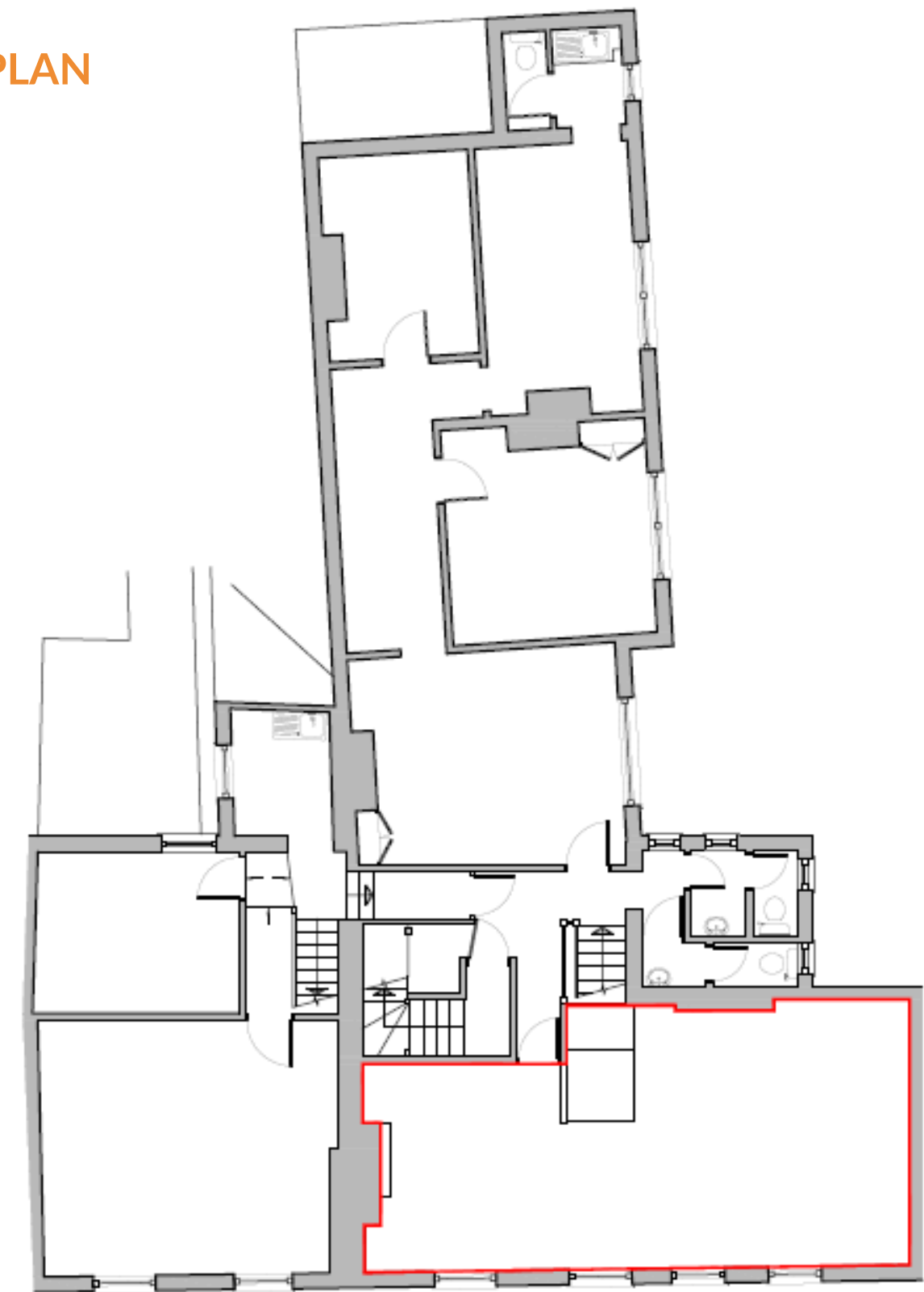
First floor
